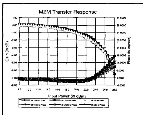
Fig. 2. MZM measured transfer response at Ku-band.
