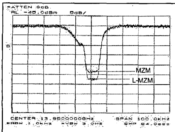
Fig. 10. NPR improvement with L/MZM at 6 dB OPBO.
